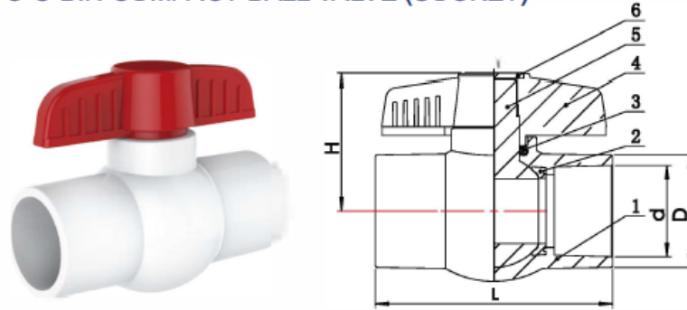
PVC-U DIN COMPACT BALL VALVE (SOCKET)
